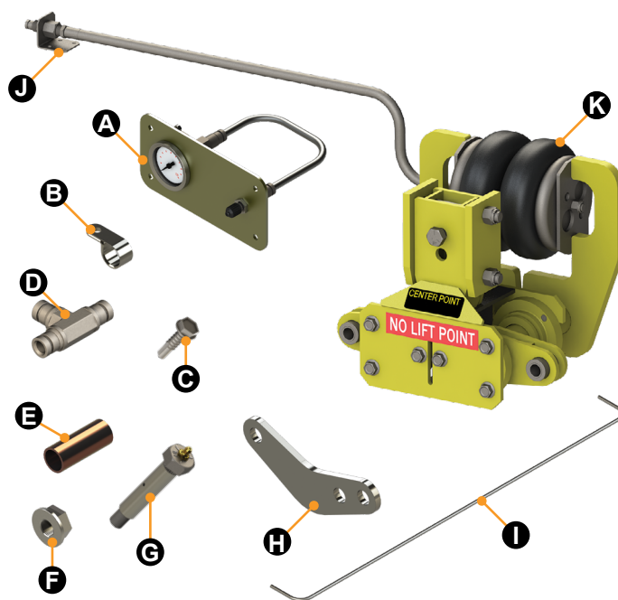
Center Point Tandem Axle Kit Part # 1565391
